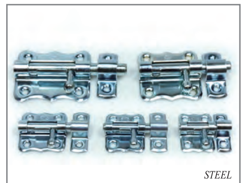
SDB8221 25mmL x 33mmW, 30L x 33W, 35L x 34W, 40L x 39W, 50L x 47W, 60L x 49W
